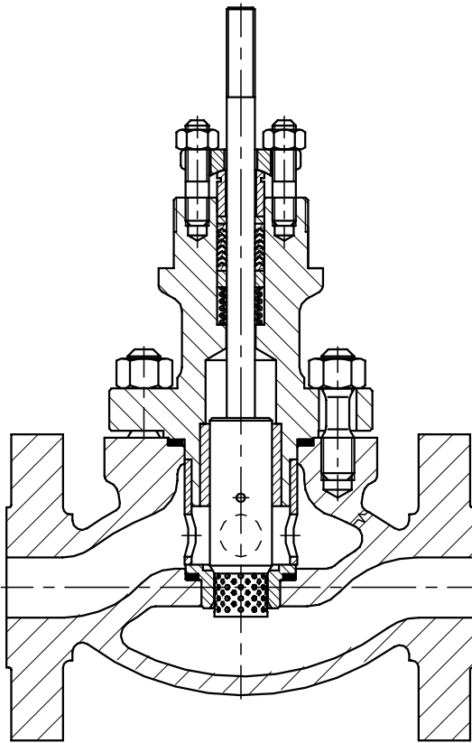
Fig. 1c. Valve S1A - perforated valve plug and compression cage.
