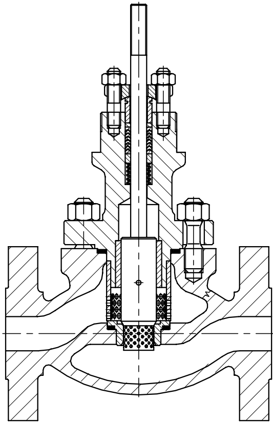
Fig. 1d. Valve S1A - perforated valve plug and choke cage
