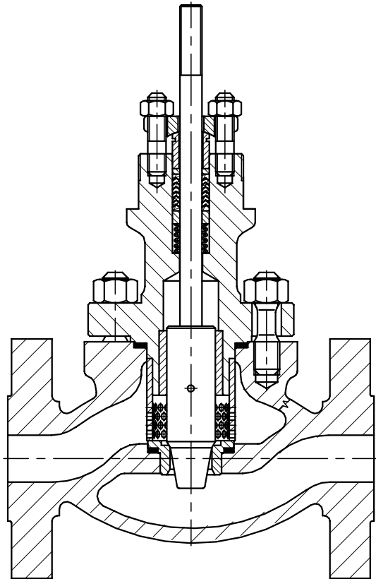
Fig. 1b. Valve S1A - contoured valve plug and choke cage
