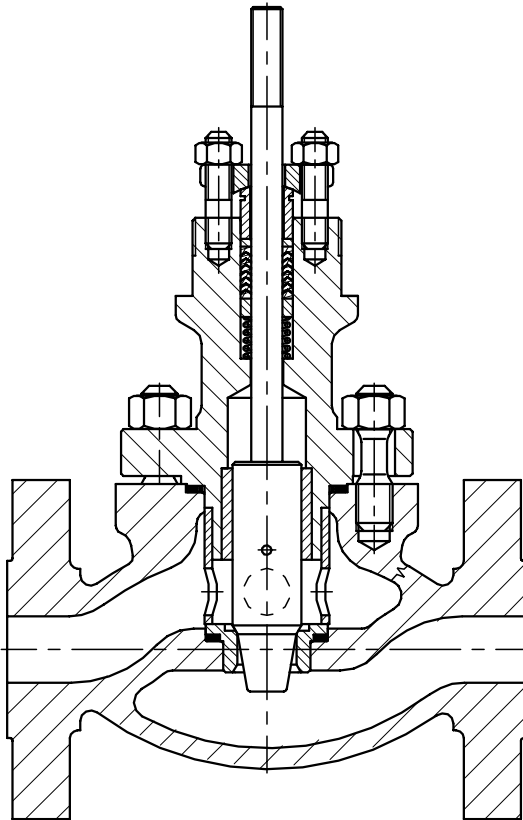
Fig. 1a. Valve S1A - contoured valve plug and compression cage
